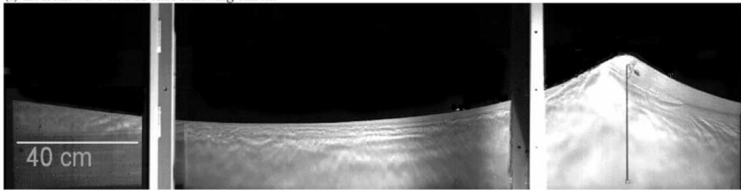
(b) the freak wave on a -10 cm/s opposing current
